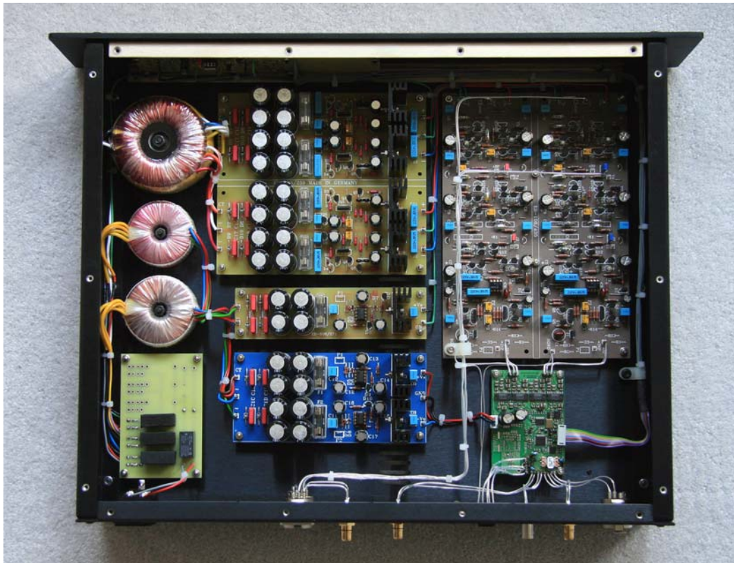
FET 435-259 Parallel DAC Interior
