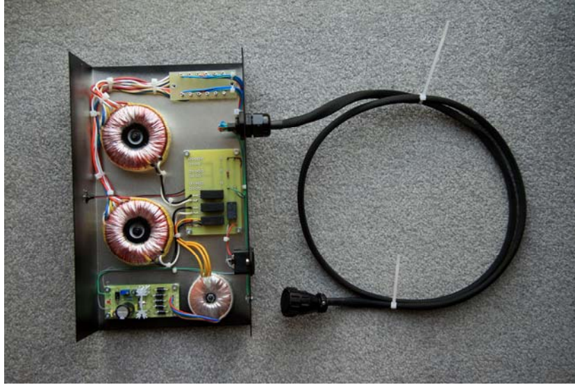
Balanced All-FET 325-259 Power Supply Interior
