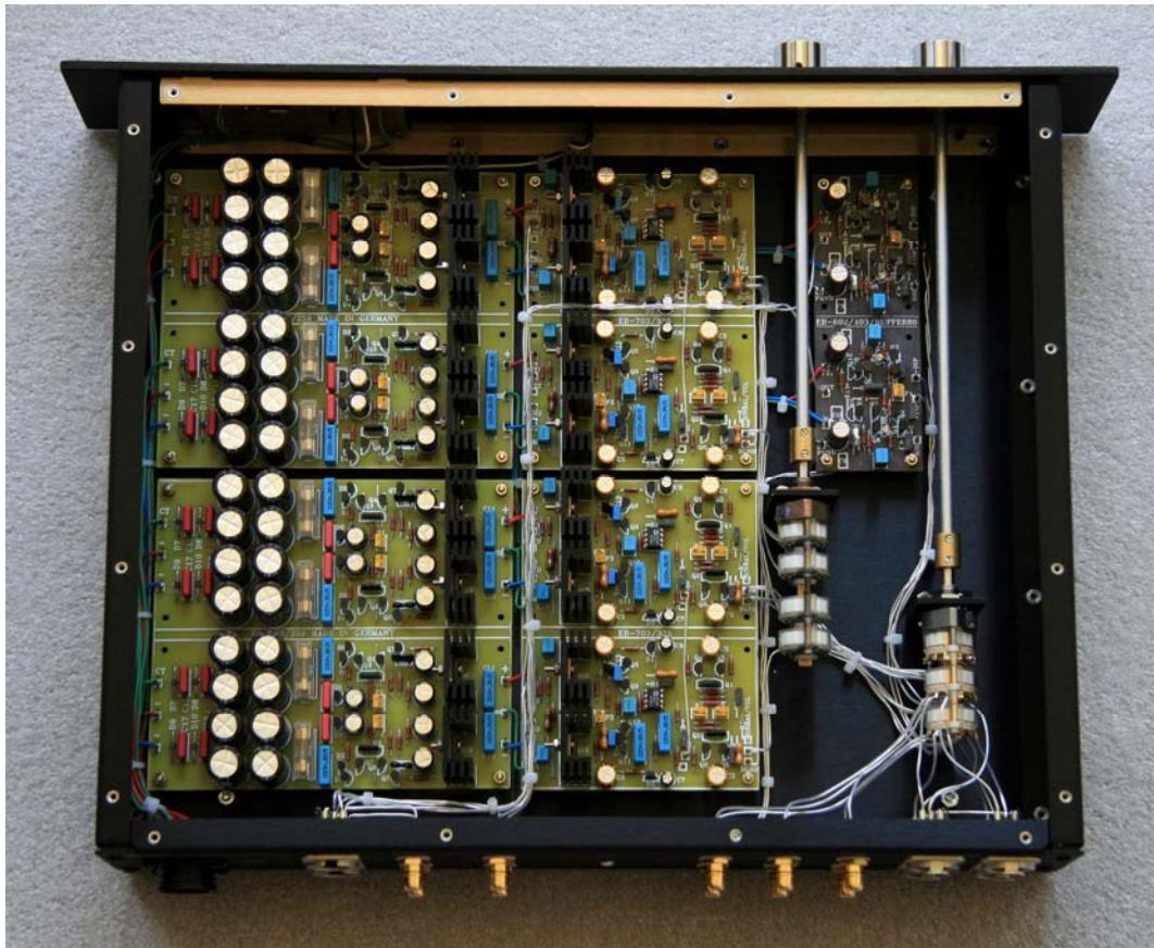
Balanced All-FET 325-259 Line Amp DACT volume control, ELMA input switching
