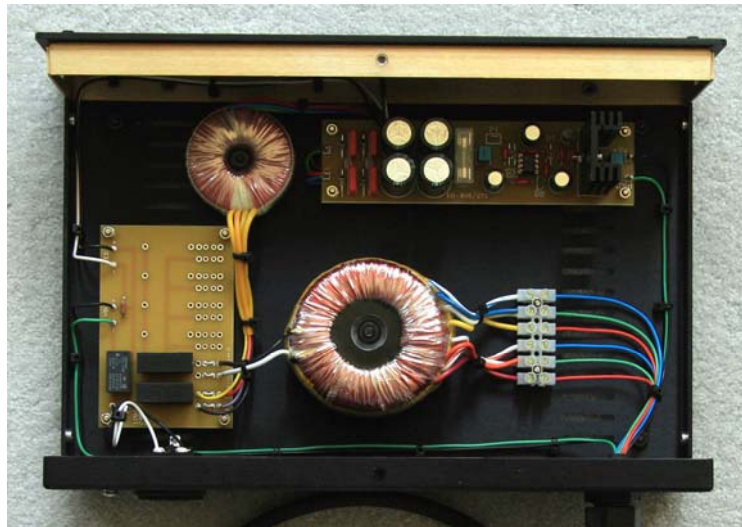
All-FET 325-259 Power Supply Interior
