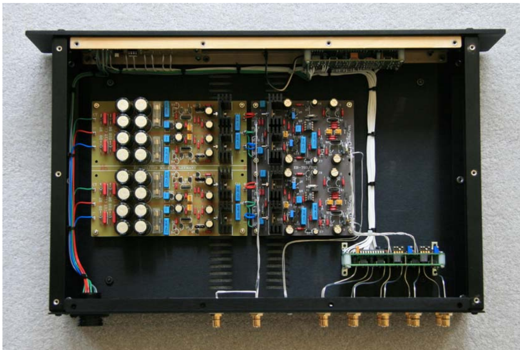
All-FET 325-259 Line Amp with Welborne Input Selector and Remote Control
