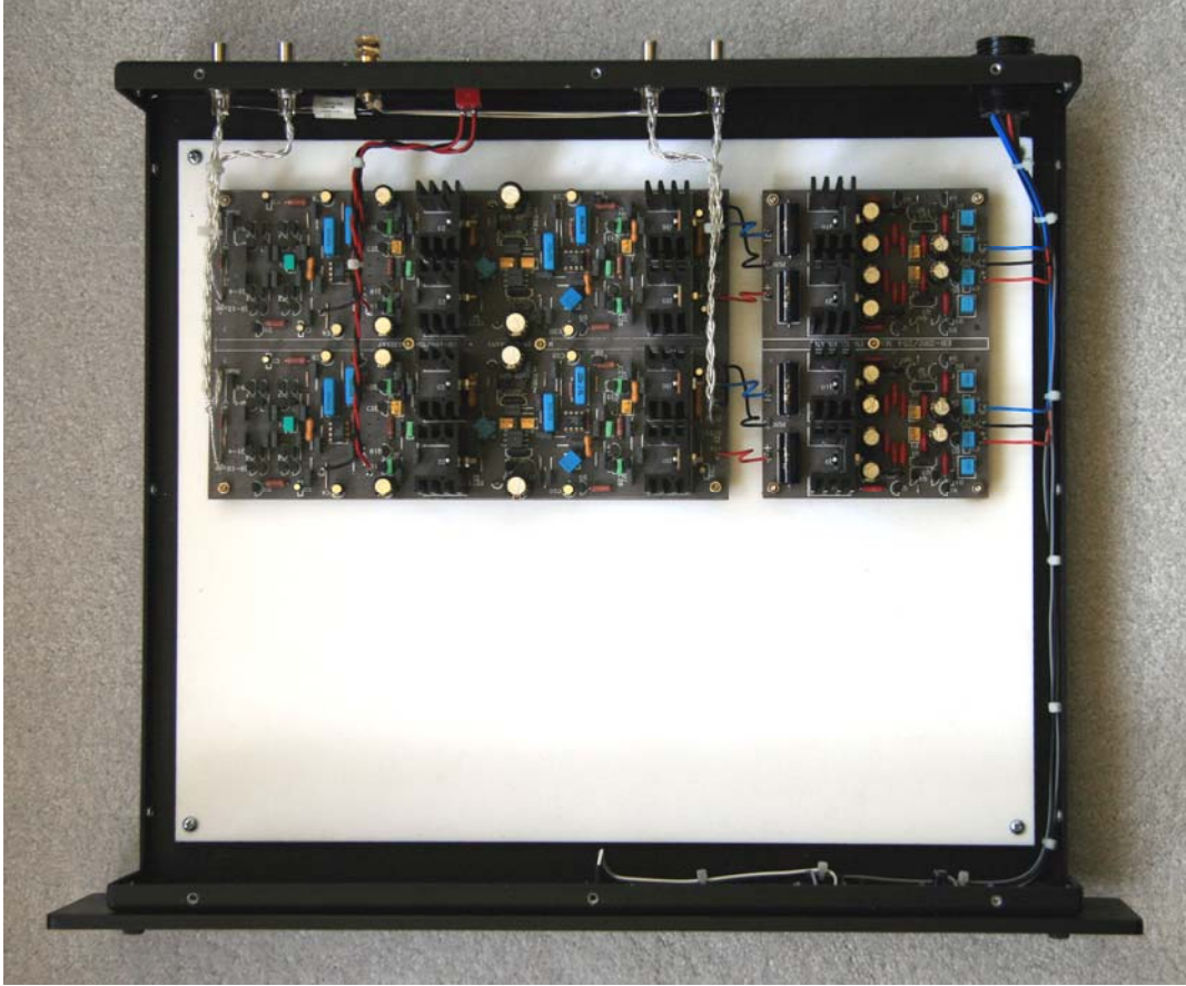
All-FET 320-254 Phono Preamplifier Interior
