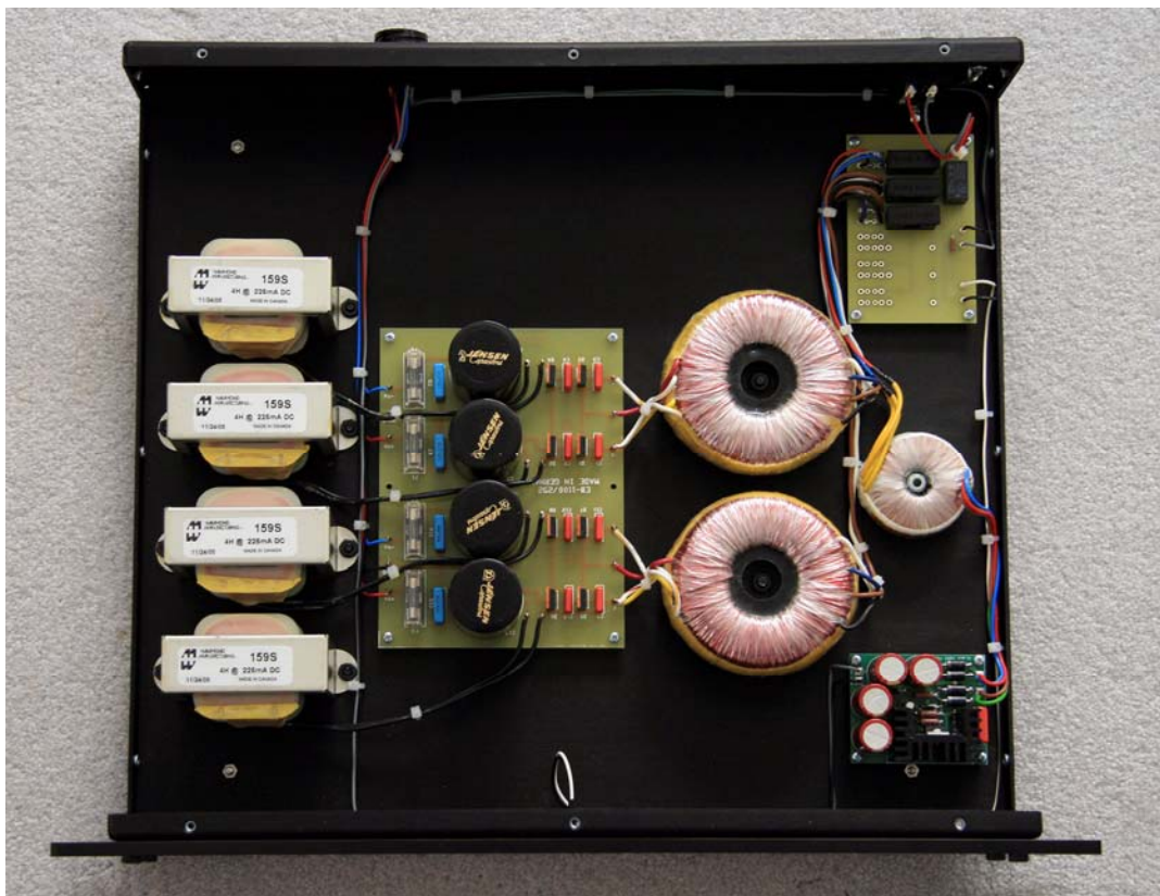
All-FET 320-254 Power Supply Interior
