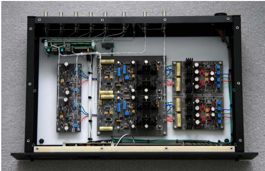
All-FET 309-254 Line Amp with Welborne Input Selector and Remote Control
