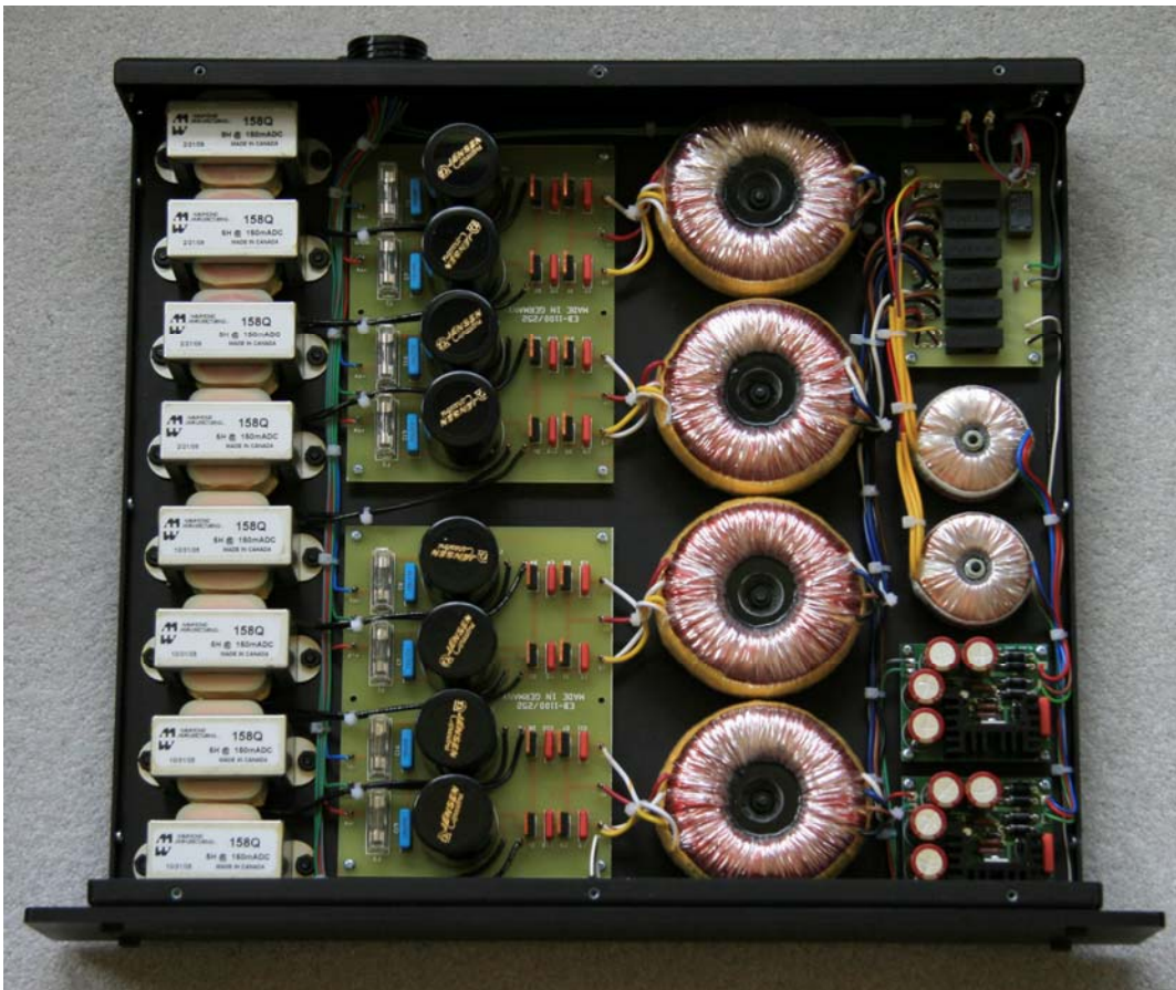
Balanced All-FET 309-254 Power Supply Interior
