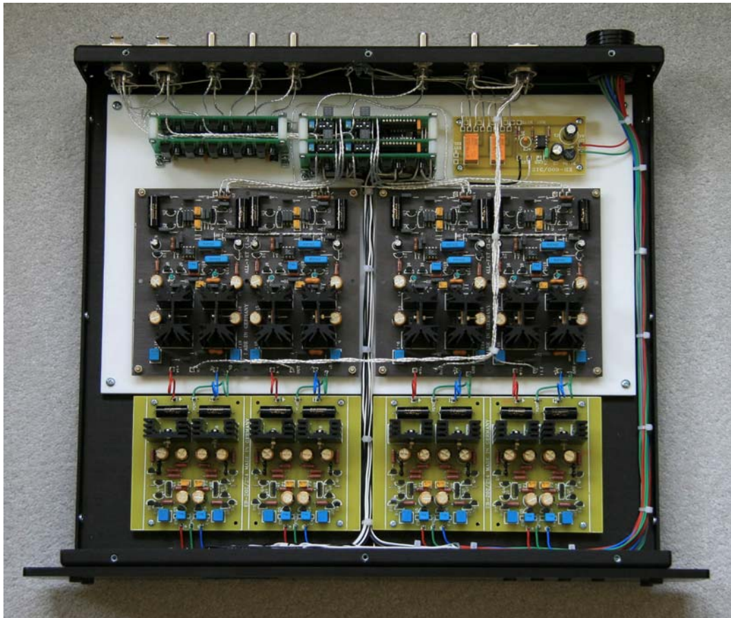
Balanced All-FET 309-254 Line Amp with Welborne Labs Remote Selector/Attenuator
